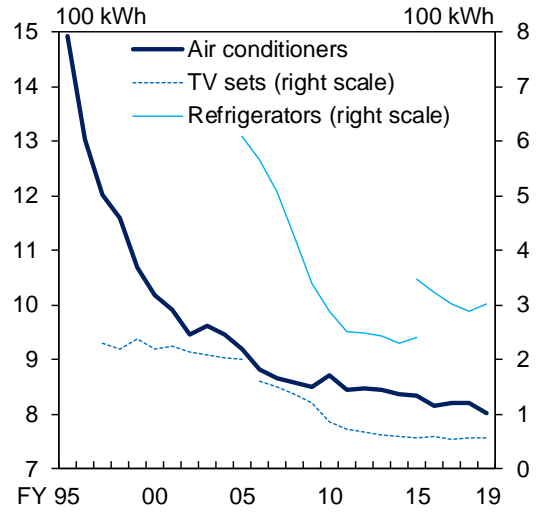
Chart 12. Energy consumption of household electrical appliances
